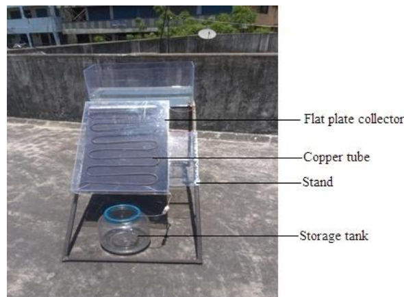
Figure 3. Experimental setup
