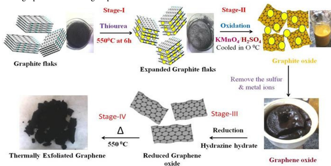
Fig.-1: Thermally exfoliated graphite to grapheme
