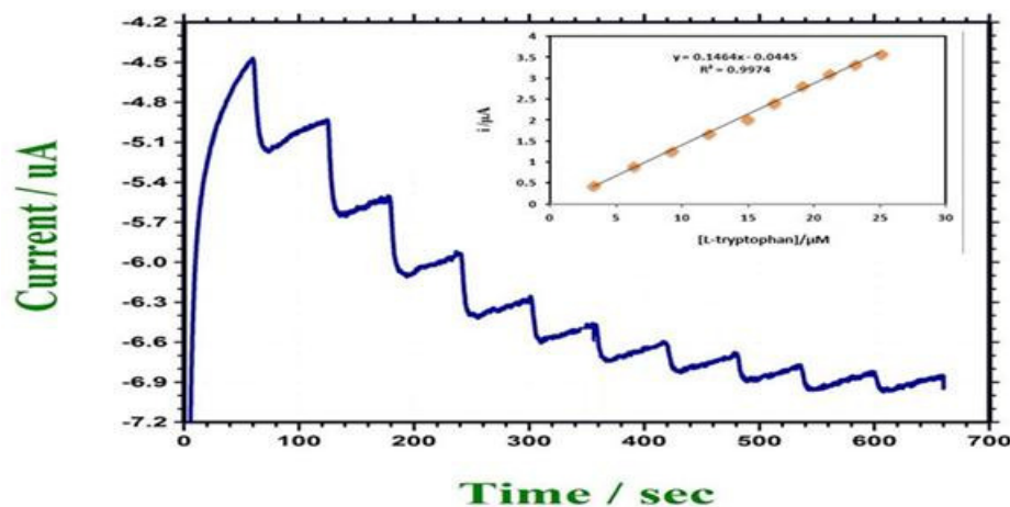
Fig.-6(A) Amperometric of steady-state catalytic current time reaction of the TEG/GCE with a following injection of L-Trp in the dynamic condition in phosphate buffer saline solution, at a fixed potential of +0.60 V. and (B) Insert the calibration plot of conc. L-Trp Vs peak current.
