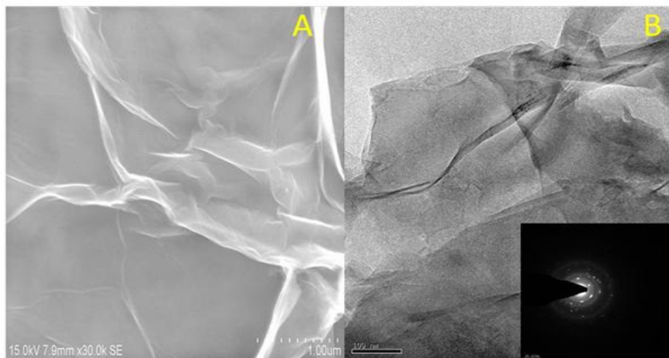
Fig.-3: (A) FESEM and (B) TEM image of thermally exfoliated graphene (insert into SAED pattern)
