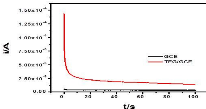
Fig.-8: Amperometric studies of the bare GCE and TEG/GCE with L-Trp in the dynamic condition in phosphate buffer saline solution.
