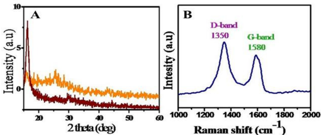
Fig.-2: (A) XRD pattern of graphene oxide and reduced graphene oxide, (B) Raman spectrum of reduced graphene oxide.
