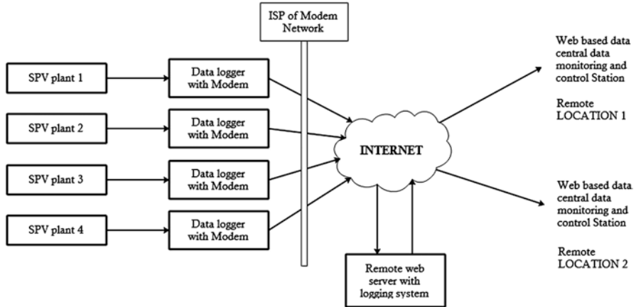
Fig. 15.4 Complete schematic of the smart remote monitoring system [7]
