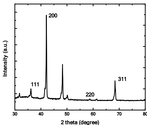
Fig.4 XRD pattern of SNA
