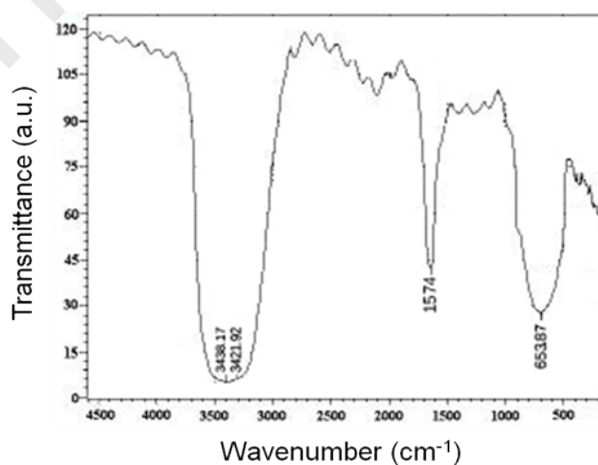
Fig.5 FTIR analysis of SNA
