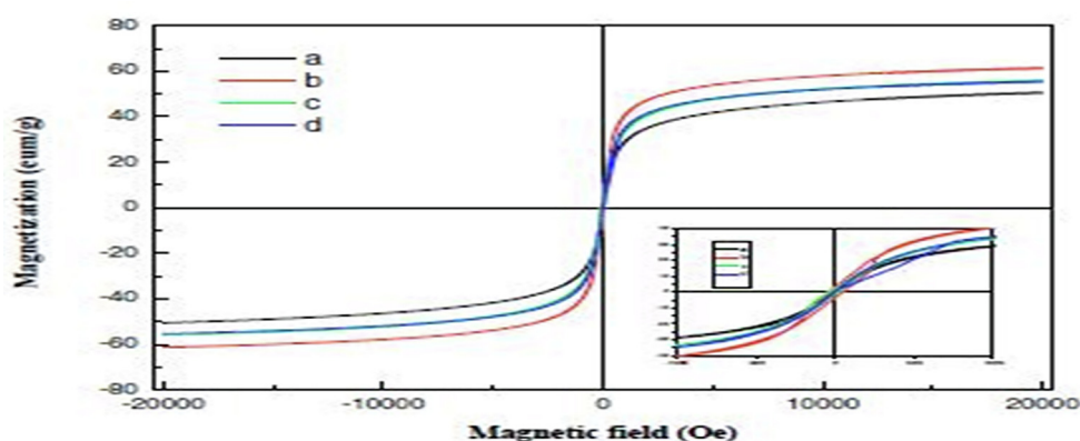
Fig. 5. Hysteresis curve of the samples.
