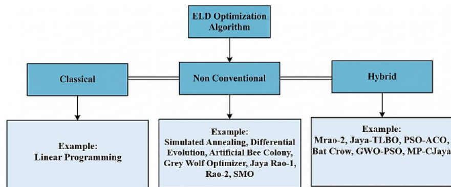
Figure 4. Optimization types
