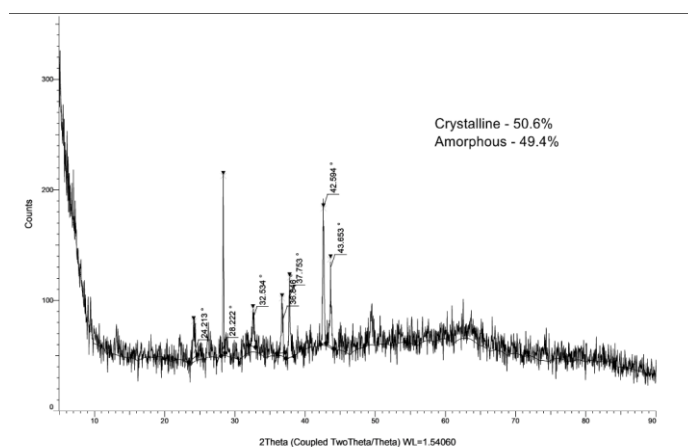
Fig. 6. XRD pattern of SeNPs
