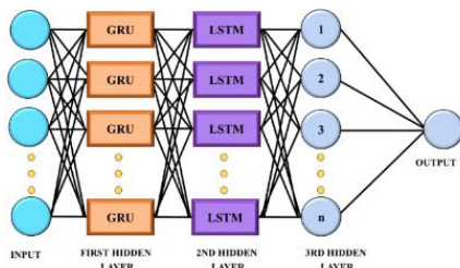
Fig. 3. Architecture diagram of GRU-LSTM
