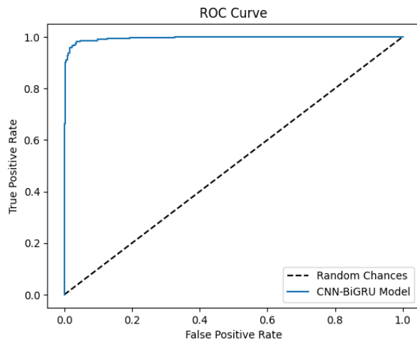
Figure.17. ROC curve
