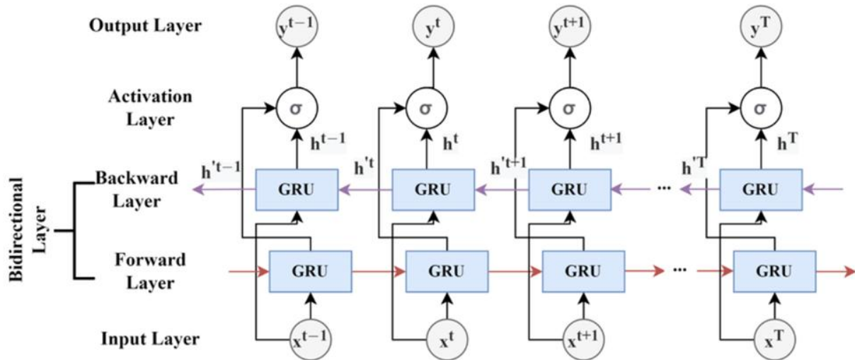
Figure.12 Architecture of Bi-GRU
