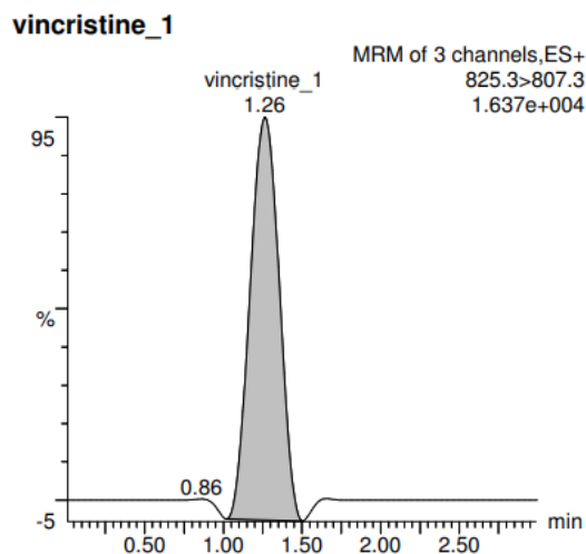
Figure 7. Chromatogram showing the amount of vincristine released on the 3 rd day in the release kinetics study of DES
