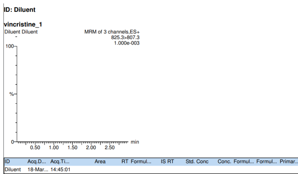
Figure 4. Chromatogram of the solvent after injecting vincristine sample
