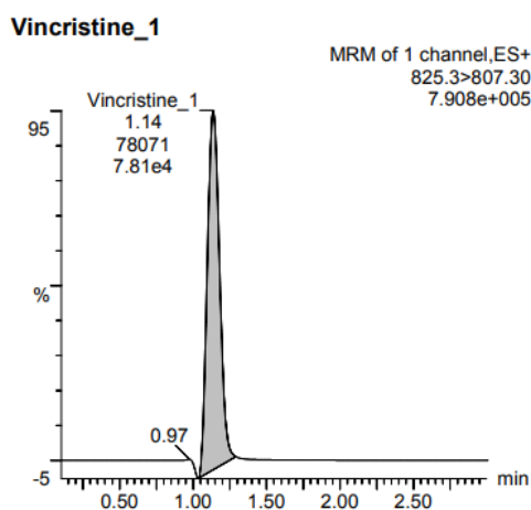
Figure 5. Day-2 inter-day precision for vincristine
