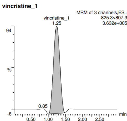
Figure 6. Chromatogram showing the amount of vincristine loaded on the DES
