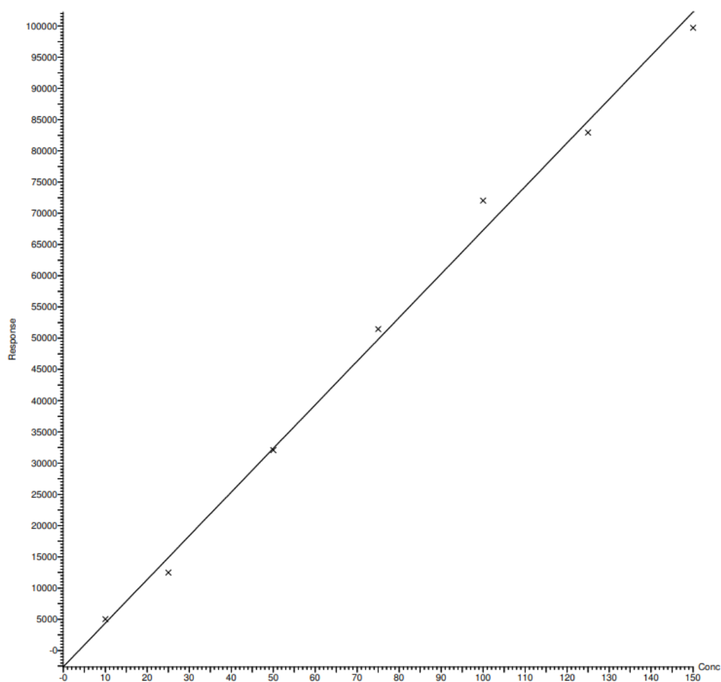
Figure 3. Linearity plot for vincristine
