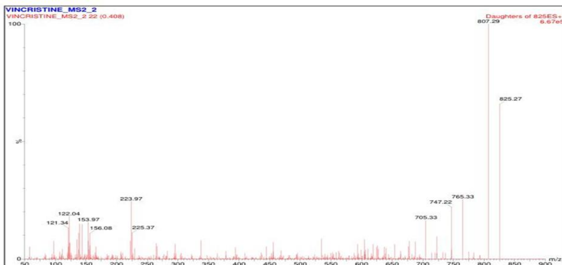
Figure 1. Molecular ion and product ions of vincristine
