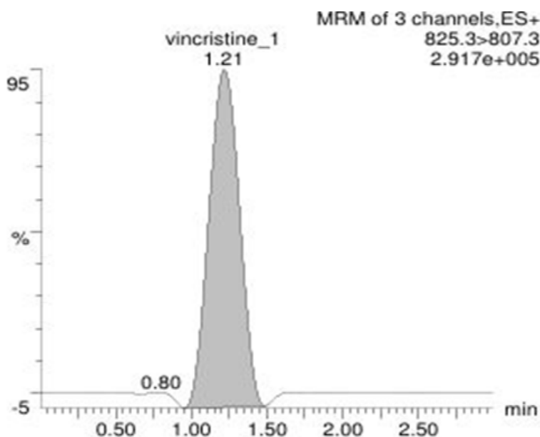
Figure 1. Molecular ion and product ions of vincristine
