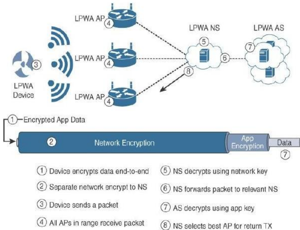
Figure 2.11 LoRaWAN Security
