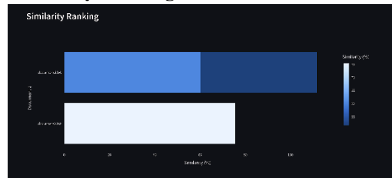
Similarity Ranking
