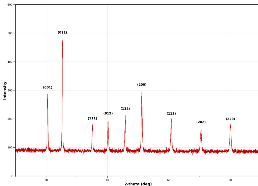
Fig. 16. X-ray diffraction (XRD) pattern of metal alkali caesium carbonate nanoparticles, displaying characteristic peaks at specific 2-theta values, confirming crystalline structure and phase identification of the nanoparticles.
