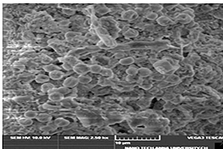
Fig. 15. Scanning Electron Microscopy (SEM) image showing the morphology of caesium carbonate nanoparticles, revealing a granular structure with spherical and irregularly shaped particles at 2.50\text{k}\times magnification. Scale bar: 10\ \mu\text{m} .
