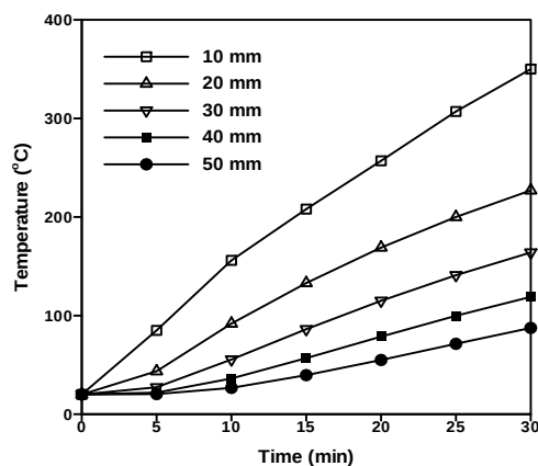
Figure 4 Time Vs. Temperature
