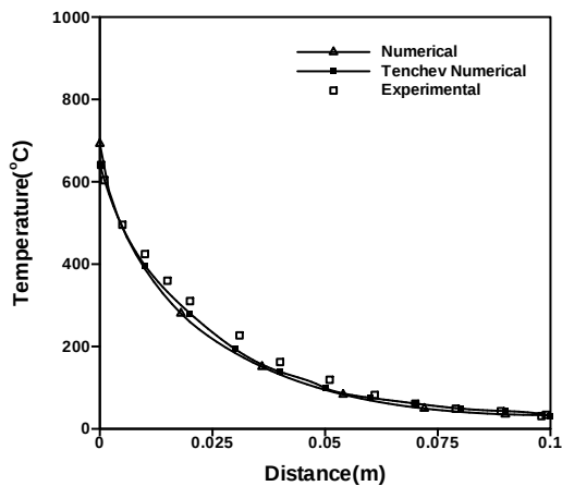
Figure 2 Temperature distribution at the end of 30 minutes
