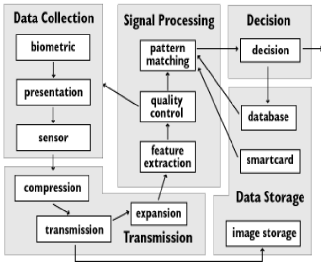
Figure 1:Biometric System
