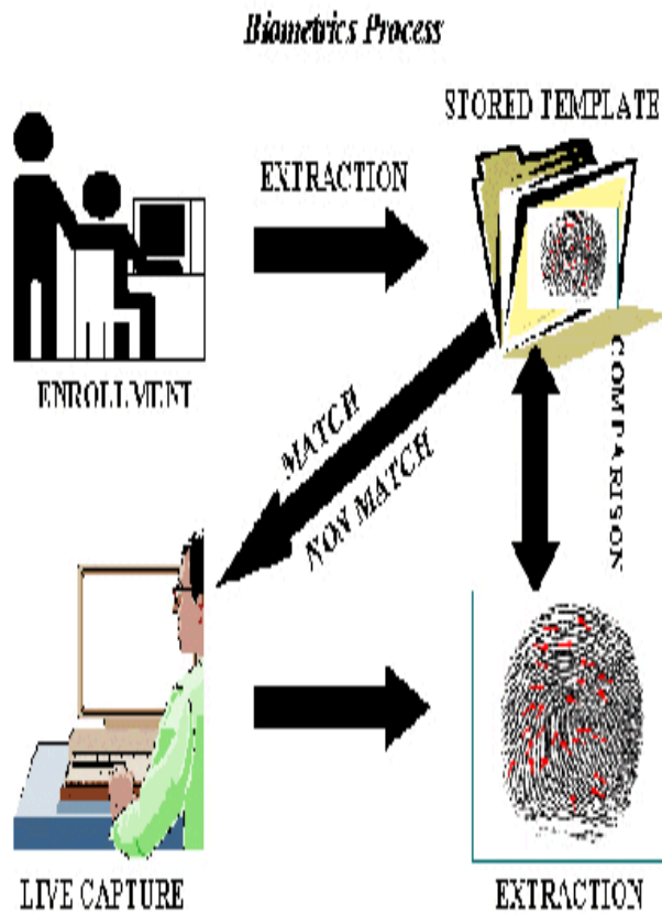
Figure2: Biometric Process
