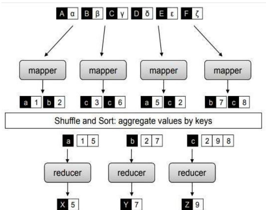
Fig 3.1: Shuffle and Sort: Aggregate Values by Keys
