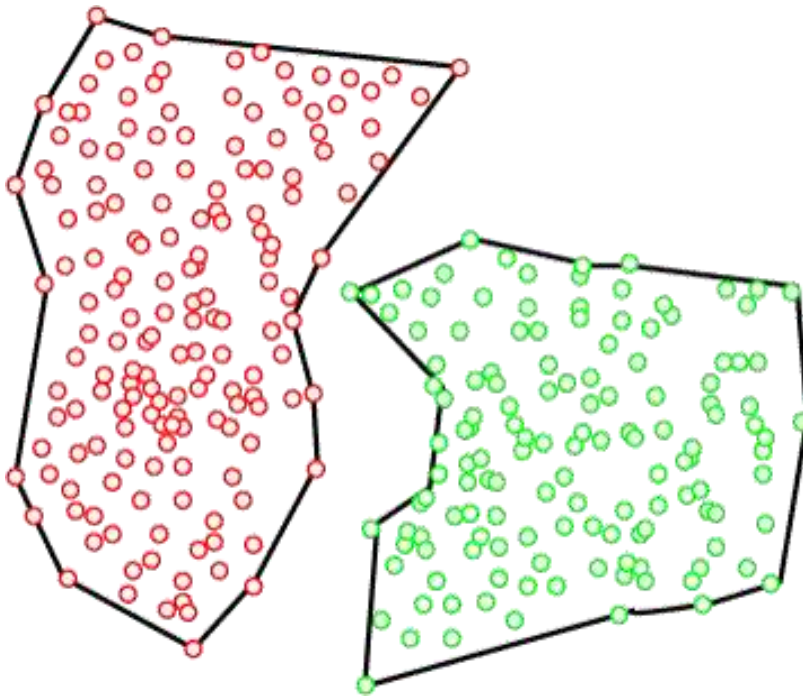
Fig 5.3: Density-Based Clustering
