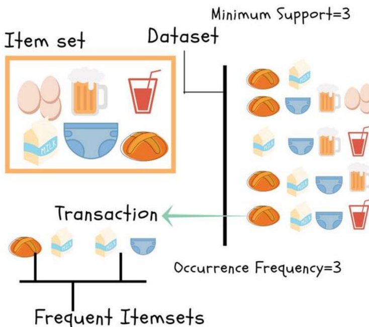
Fig 5.7: Occurrence Frequency
