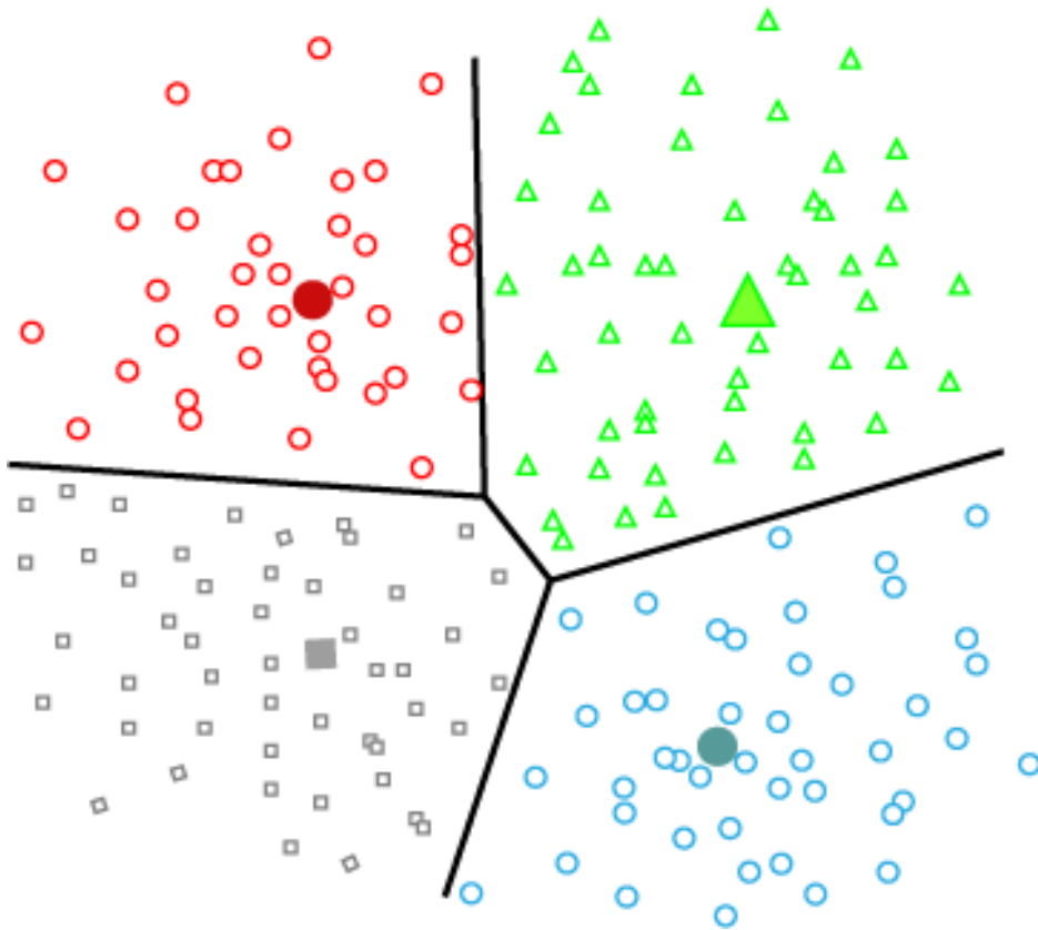
Fig 5.2: Partitioning Clustering
