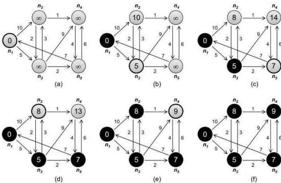
Fig 3.3: Graph Algorithms
