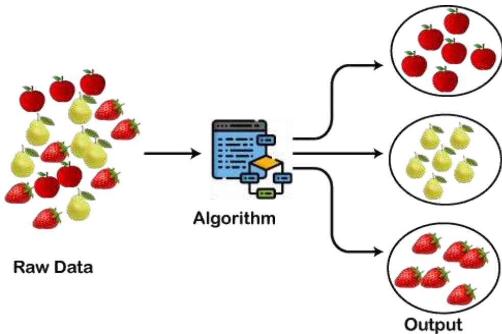
Fig 5.1: Algorithm
