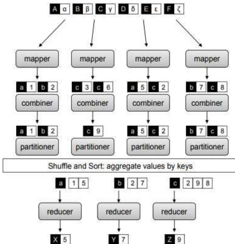
Fig 3.2: Map Reduce Basics
