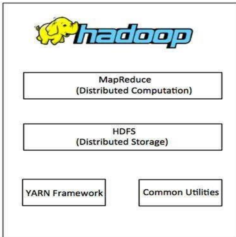
Fig 2.2: Hadoop
