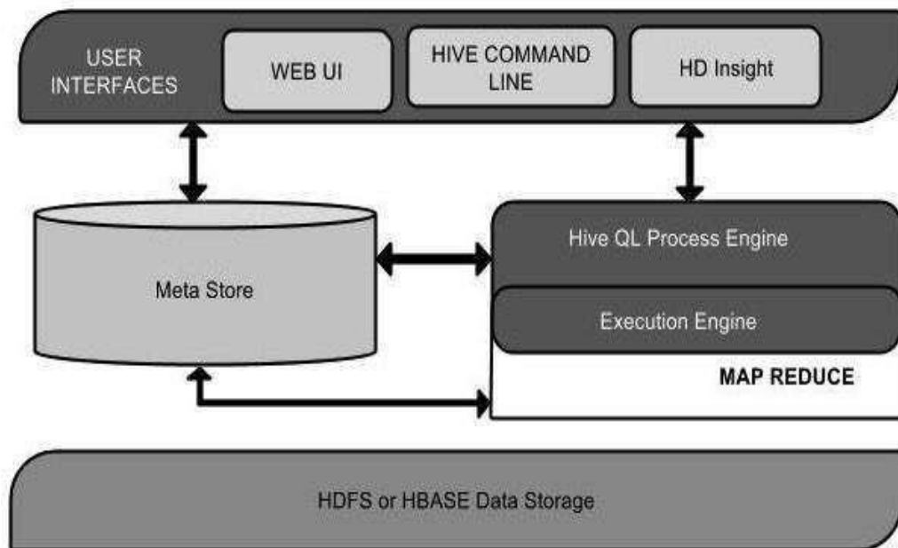
Fig 4.1: Map Reduce
