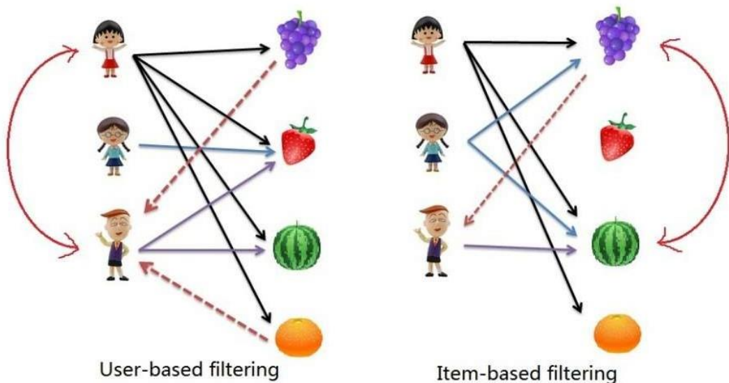
Fig 5.5: Collaborative Filtering with R
