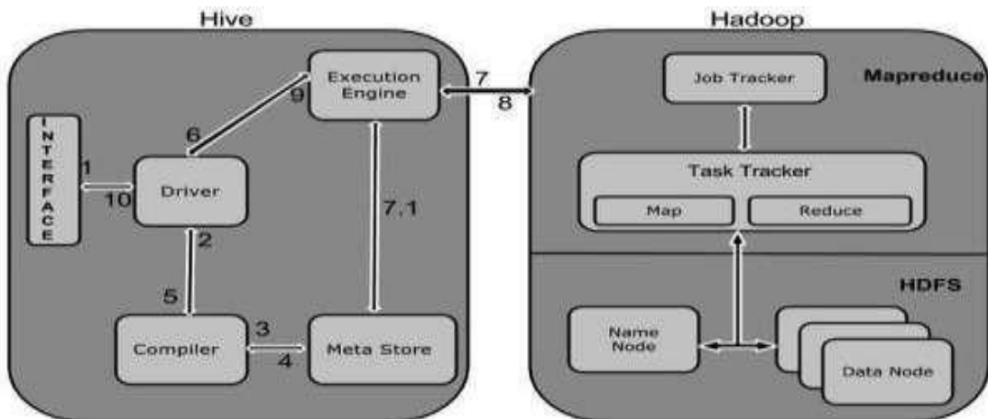
Fig 4.2: Working of Hive
