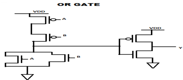
Fig. 3.2: OR Gate Circuit.
