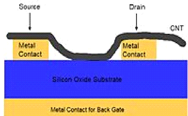
Fig. 2.2: Side View of Carbon Nanotubes Deposited on A Silicon Oxide Substrate Pre-Patterned with Source and Drain Contacts.
