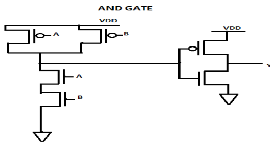
Fig. 3.1: AND Gate.
