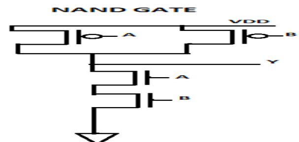
Fig. 3.3: NAND Gate.
