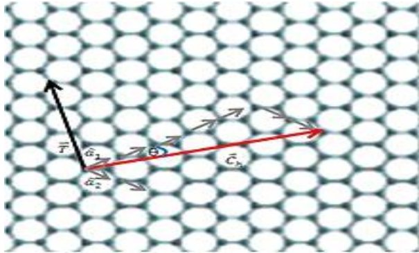
Fig. 2: Graphene Atomic Structure with A Translational Vector \vec{T} and A Chiral Vector \vec{C}_h of A CNT.
