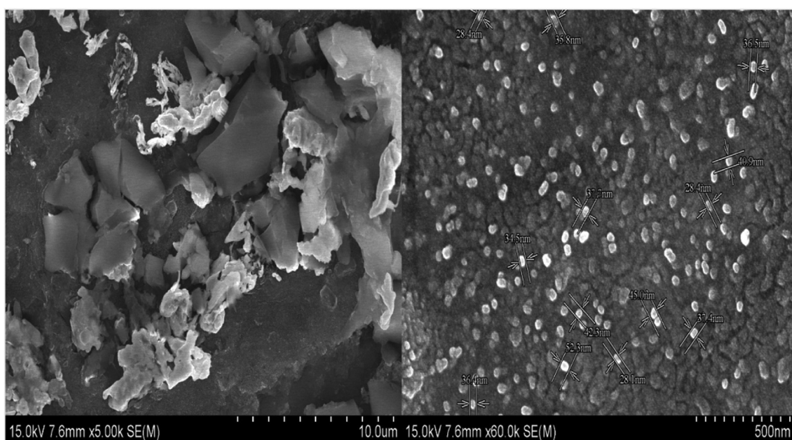
Fig. 2. FESEM images of a) Peel extract and AgNO 3 b) CPE-AgNPs with average size of 38.2 nm.
