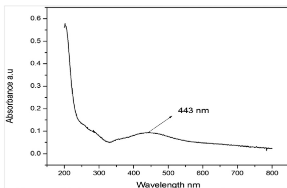
Fig. 3. UV-Visible spectra of CPE-AgNPs.
