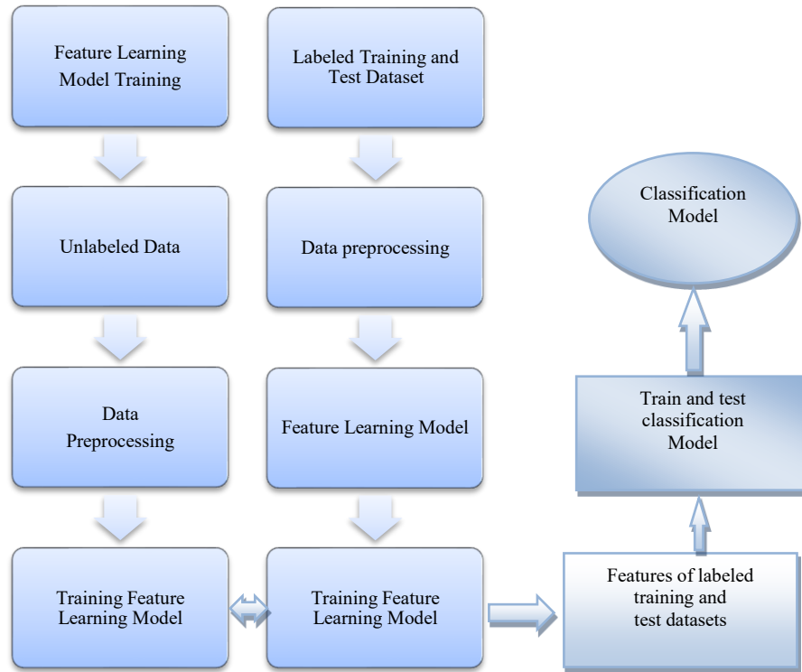
Fig. 2 Fraud detection process for financial fraud
