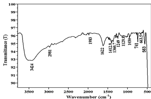
Fig. 7 — FTIR graph in green synthesis of NiO nanoparticle using Vn leaf extract
