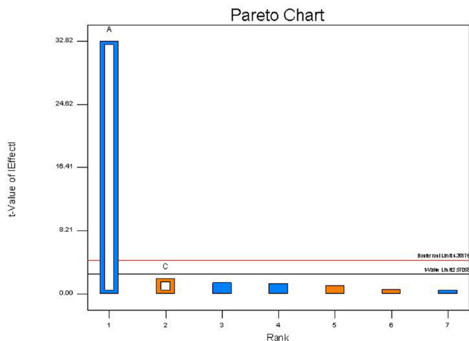
Figure 2. A Pareto chart showing effects of influential critical process attributes on first response, R_t (retention time).
