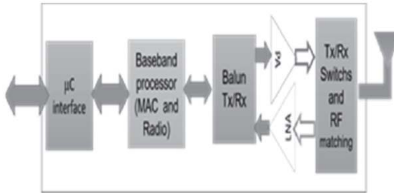
FIGURE 3. Block diagram of the Wi-Fi module
