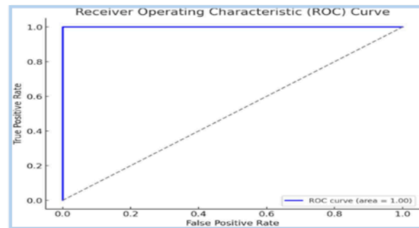
Fig. 6: ROC Curve.
