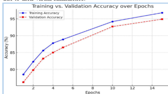
Fig. 1: Training vs. Nalidation Accuracy Over Epochs.
