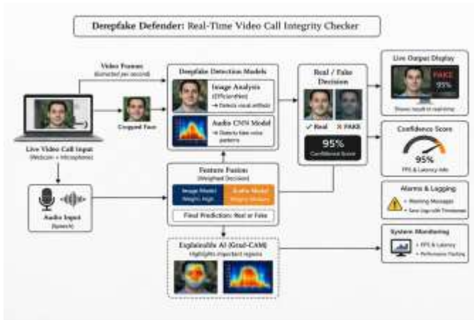
Fig. 1. DEEFAKE ARCHITECTURE DIAGRAM
