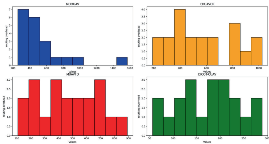
Figure 16. Routing overhead
