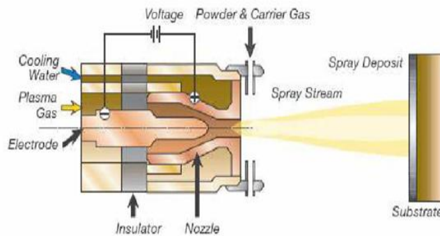
Fig.3 (a) Plasma spray gun cross section.
