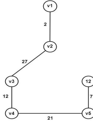
Figure 5. Antenna graph of decrypted adjacency matrix.
