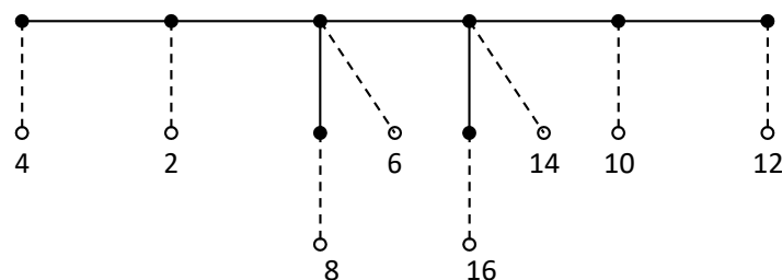
Figure 4: Corona Tree T \odot K_1 with all even labeled vertices as defined in Equation 1
