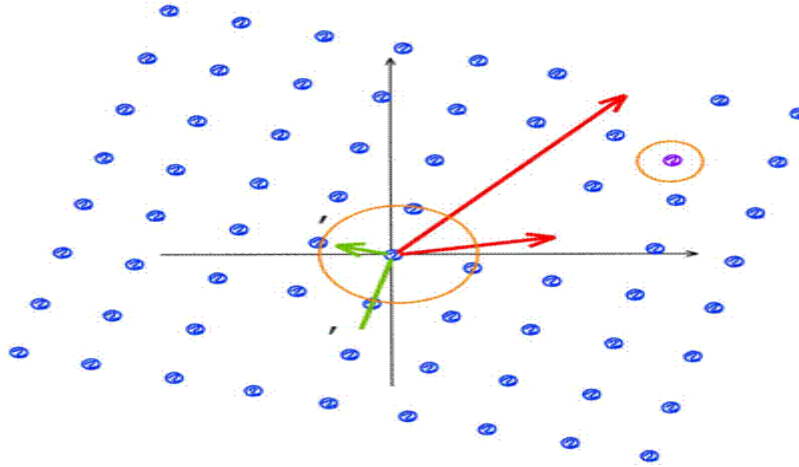
Figure 2: Illustration of a 2-Dimensional lattice
