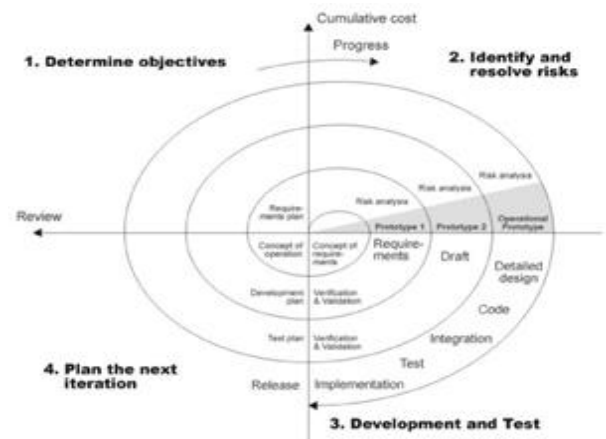
Fig. 3: Spiral Model [6].
