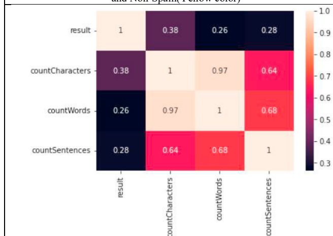
Fig. 5. Heat map to visualize the dataset with character count, word count and sentence count.
