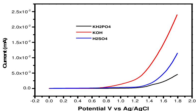
Fig.-2: LSV of the bare electrode in with 0.5\text{ M} potassium dihydrogen phosphate, 0.5\text{ M} of sulphuric acid and 1\text{ M} of Potassium Hydroxide solution at a scan rate of 5\text{ mV/sec} .
