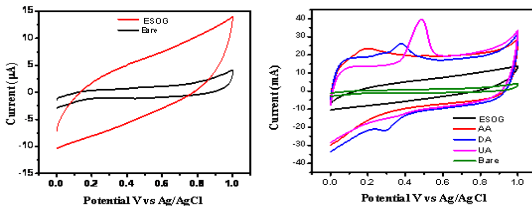
Fig.-4(a): CVs of bare and ESOG in 0.1M PBS (pH.7.2) at scan rate of 50 mV/sec.
