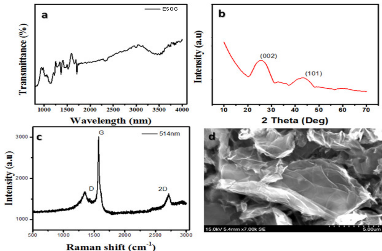
Fig.-3: FTIR,XRD, Raman Spectroscopy,SEM.
