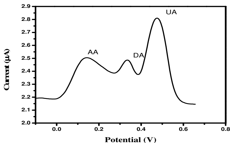
Fig.-6: DPV result of 1 mM AA, 0.5 mM DA and 1 mM UA in 0.1 M PBS solution (pH 7.2) on ESOG at 50 mV pulse amplitude.
